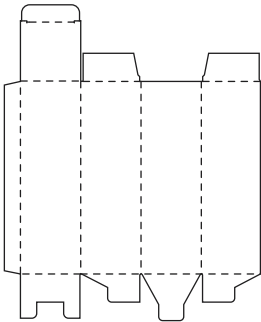
OPTIONAL BOX 240 x 75 x 75 mm SCALE (1:2)
